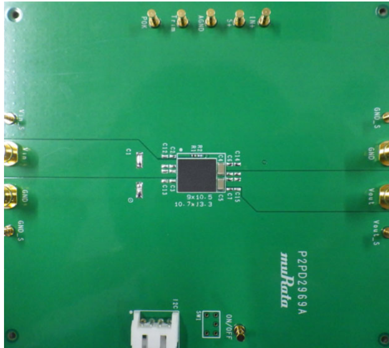
Figure 34. Applicatuin Board Example (Based on JEDEC standard) 114.5 × 101.5 × 1.6mm (4 Layer FR-4) Outside copper(1,4) layer=2oz, Inner copper(2,3) layer=1oz
