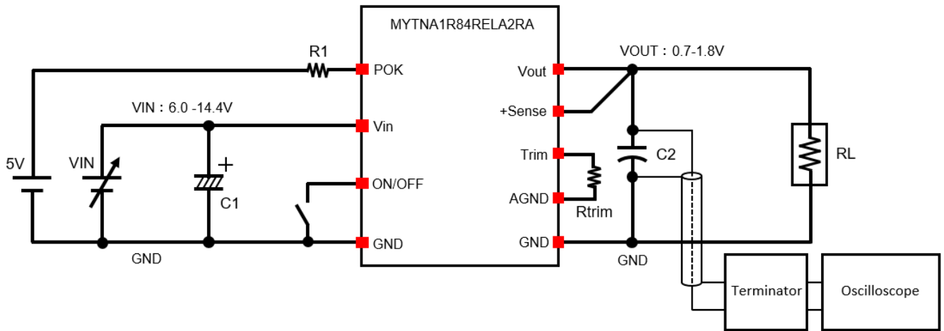
Figure 29. Test Circuit
